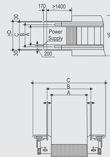
↑ SKIRTING BRUSH
